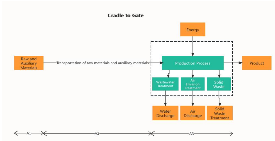
Figure 2: System diagram
