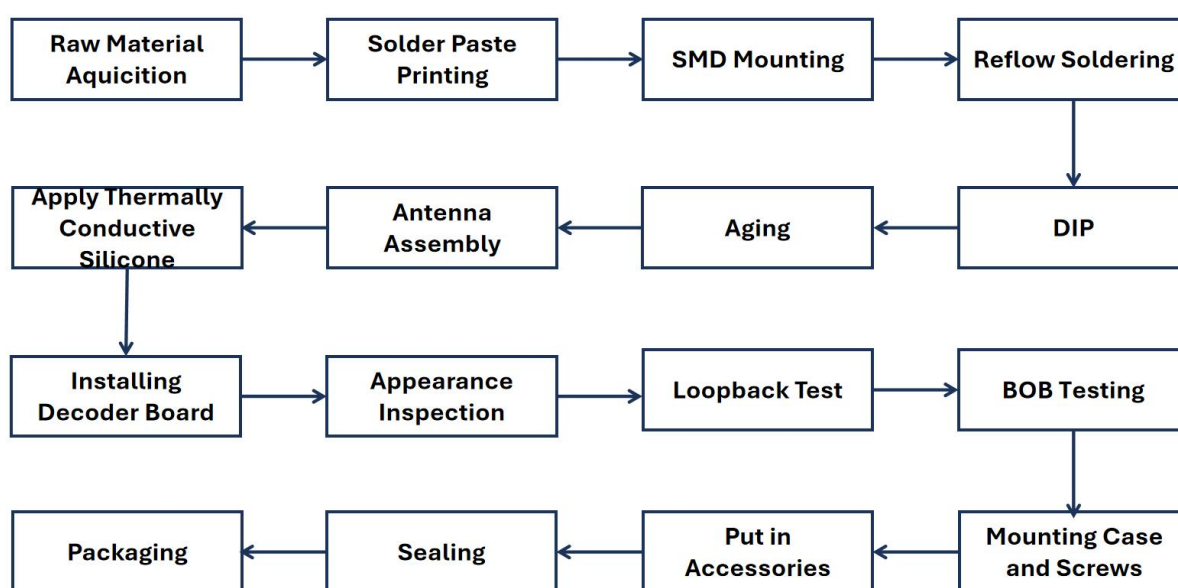
Figure 4: The production process flow of TIM HUB Pro, GPON ONT-ZXHN F6745M
