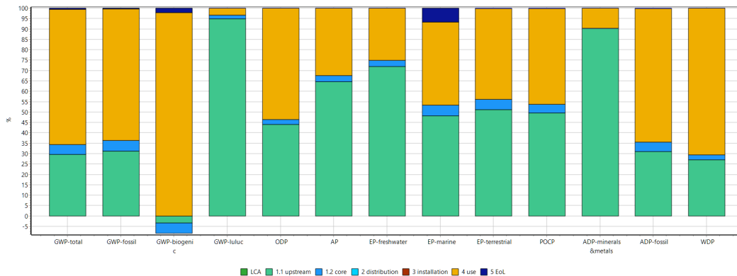
Figure 4 Life cycle contribution analysis of EMC300 MV metering system
